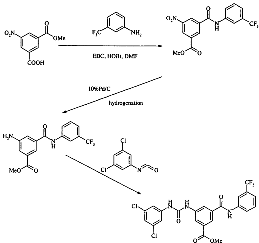
Scheme III-B
